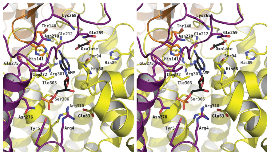
Figure 5 Stereoview of the active site. A molecule of AMP is bound in the active site formed by regions of three of the four subunits. There are four active sites per tetramer, with each active site formed by contributions from three of the four subunits, in this case by A (yellow), B (orange) and D (purple). The same colour scheme is used as in Fig. 2.
