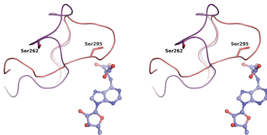
Figure 7 Stereoview of the different conformations displayed by the active-site loop. The SaPurB structure is shown in purple and the E. coli enzyme structure is shown in pink. The adenylosuccinate is depicted as in Fig. 6.
