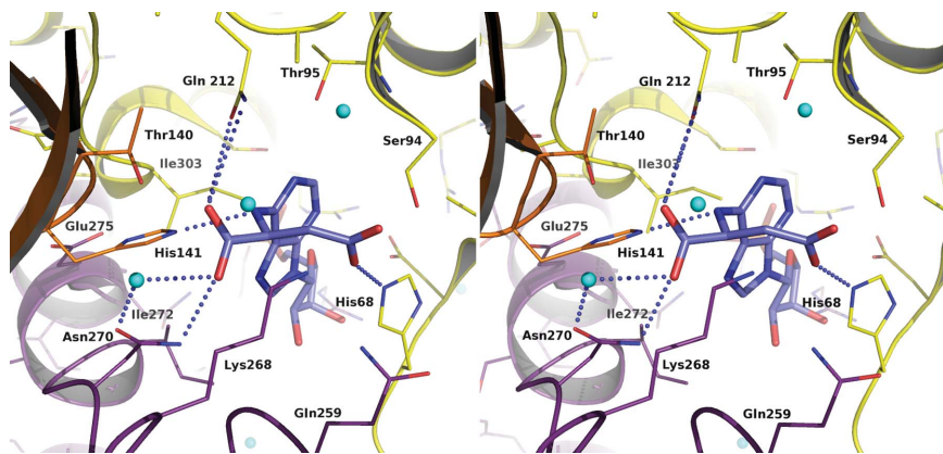
Figure 6 Stereoview of the adenylosuccinate model in the active site of SaPurB . The colour scheme is the same as that used in Fig. 2, except that the C atoms of the ligand are shown in light blue.
